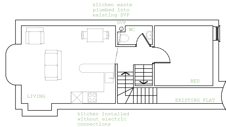
FIRST FLOOR PLAN AS EXISTING
