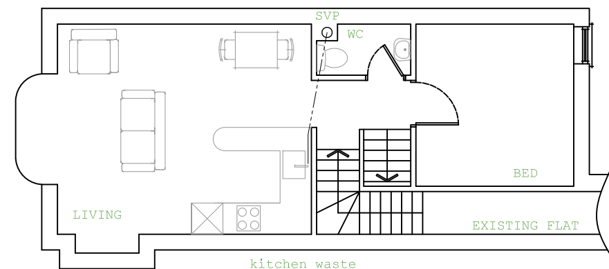
FIRST FLOOR PLAN AS PROPOSED
