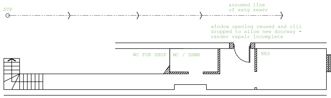
GROUND FLOOR PLAN AS EXISTING
